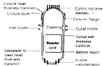
Typical PWR vessel showing important degradation sites
