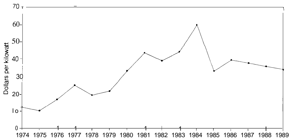
Figure 3-10—Average Annual Nuclear Power Plant Capital Additions Costs 1974-1989 (1991 dollars per kilowatt of capacity)
