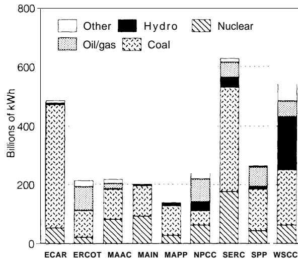
Figure 3-3—U.S. Regional Electricity Supplies by Fuel, 1991
