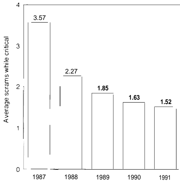
Figure 2-4—Average Number of Reactor Scrams While Critical
